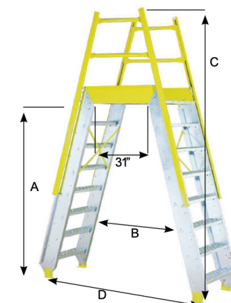
Ship's Ladder Crossover Bridge
