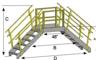
Stair Crossover Bridge
